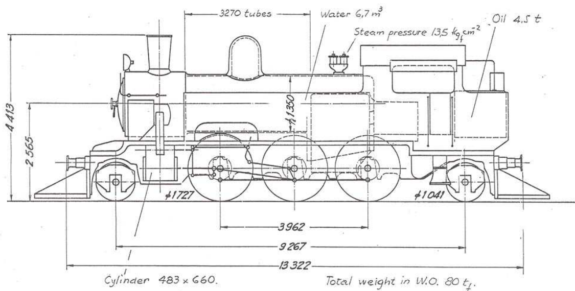
Fig. 2: Locomotive N°3477, prototype class ROBC2, FCGR, Argentina. Built in 1915, modernized by the author in 1954. Drawbar power: 1400 HP.
