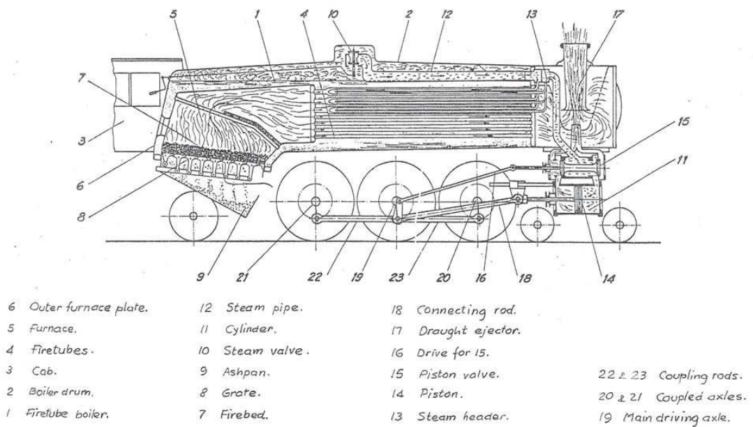
Fig. 10: Essential components of a traditional 1914 steam locomotive.
